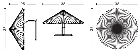
MATIN WALL 380 WIDTH 38 CM | 14.96" DEPTH 25 CM | 9.84" HEIGHT 38 CM | 14.96"
