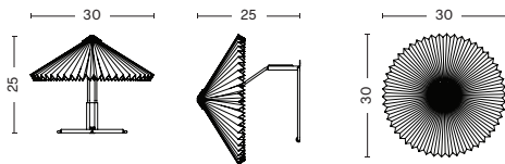
MATIN WALL 300 WIDTH 30 CM | 11.81" DEPTH 25 CM | 9.84" HEIGHT 30 CM | 11.81"
